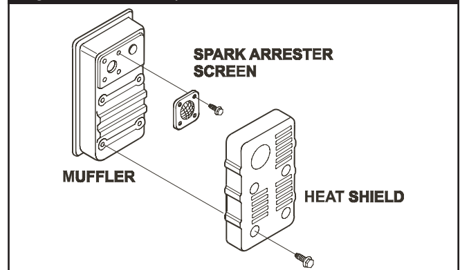
Figure 18 — Service Spark Arrester
