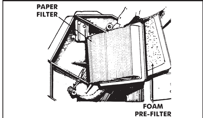
Figure 16 — Service Air Cleaner
